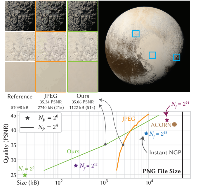
Fig. 8. We fit Compact NGP to the 8000 \times 8000px Pluto image using parameters N_f = 2^6 and N_p = 2^4 and varying N_c (green curve ranging from 2^{12} to 2^{24} ). We show that we are able to outperform JPEG on a wide range of quality levels. The qualitative comparisons at equal size (insets) show the visual artifacts exhibited by different methods: while JPEG has color quantization artifacts, ours appears slightly blurred.
