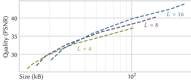
Fig. 9. Impact of the number of multiresolution levels L on PSNR vs. size. We use the parameters N_f = 2^6 and N_p = 2^4 while varying N_c (curve ranging from 2^{12} to 2^{20} ) and L on the image compression task from Figure 1. The default value L = 16 (inherited from Instant NGP) performs well for a large range of sizes, particularly in the hundreds of kB range that is most practical. Yet, a lower number of levels results in a better Pareto curve at smaller sizes that could be used if one wanted to compete with MLP based image compression techniques; cf. Figure 7.
