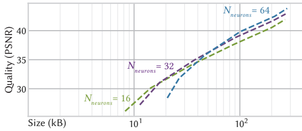
Fig. 10. Impact of the MLP width N_{\text{neurons}} on PSNR vs. size. The parameter sweeps over N_f , N_p , and N_c are the same as Figure 9. A similar conclusion can be drawn: the default value N_{\text{neurons}} = 64 (inherited from Instant NGP) performs well at practical sizes, whereas a better Pareto front can be achieved at smaller sizes.
