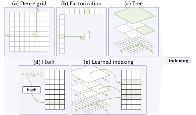
Fig. 3. Various indexing schemes mapping integer grid coordinates \mathbf{v} = (v_0, v_1, \dots) to feature vectors have been proposed, including (a) dense grids, (b) k -planes, (c) sparse grids and trees, (d) spatial hashing, and (e) learned indexing. Since each scheme ultimately computes an index into a codebook of feature vectors, the schemes can be combined by arithmetic operations on the indices they produce. Our method combines deterministic hashing and a learned indexing as visualized in Figure 4.
