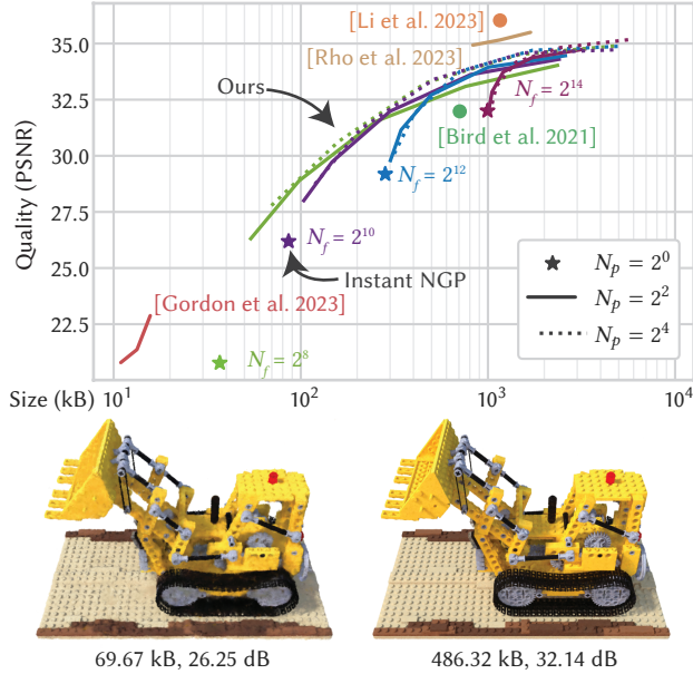
Fig. 6. PSNR vs. file size for varying hyperparameters in compressing the NeRF Lego digger. The layout is the same as Figure 5. We also show rendered images of our compressed representation at two quality settings.
