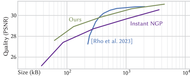
Fig. 2. Size vs. PSNR Pareto curves on the NeRF scene from Figure 1. Our work is able to outperform Instant NGP across the board and performs competitively with masked wavelet representations [Rho et al. 2023].
