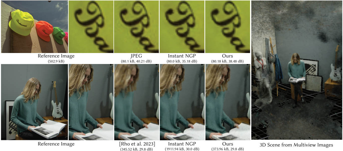
Fig. 1. Compact neural graphics primitives (Ours) have an inherently small size across a variety of use cases with automatically chosen hyperparameters. In contrast to similarly compressed representations like JPEG for images (top) and masked wavelet representations [Rho et al. 2023] for NeRFs [Mildenhall et al. 2020] (bottom), our representation neither uses quantization nor coding, and hence can be queried without a dedicated decompression step. This is essential for level of detail streaming and working-memory-constrained environments such as video game texture compression. The compression artifacts of our method are easy on the eye: there is less ringing than in JPEG and less blur than in Rho et al. [2023] (though more noise). Compact neural graphics primitives are also fast: training is only 1.2–2.6× slower (depending on compression settings) and inference is faster than Instant NGP [Müller et al. 2022] because our significantly reduced file size fits better into caches.
