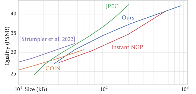
Fig. 7. PSNR vs. file size on the Kodak image dataset using parameters N_f = 2^6 and N_p = 2^4 and varying N_c (blue curve ranging from 2^{12} to 2^{20} ). On this dataset, our method performs close to JPEG at small file sizes and worse at larger ones. At small file sizes, our representation is dominated by floating point parameters like the MLP and the feature codebook. Competing methods that quantize pure MLPs perform better in this regime [Dupont et al. 2021; Strümppler et al. 2022], whereas we omit quantization for simplicity and flexibility. At visually pleasant targets ( \sim 35 dB and above) these prior works do not scale as it is difficult to train pure MLPs to such qualities.
