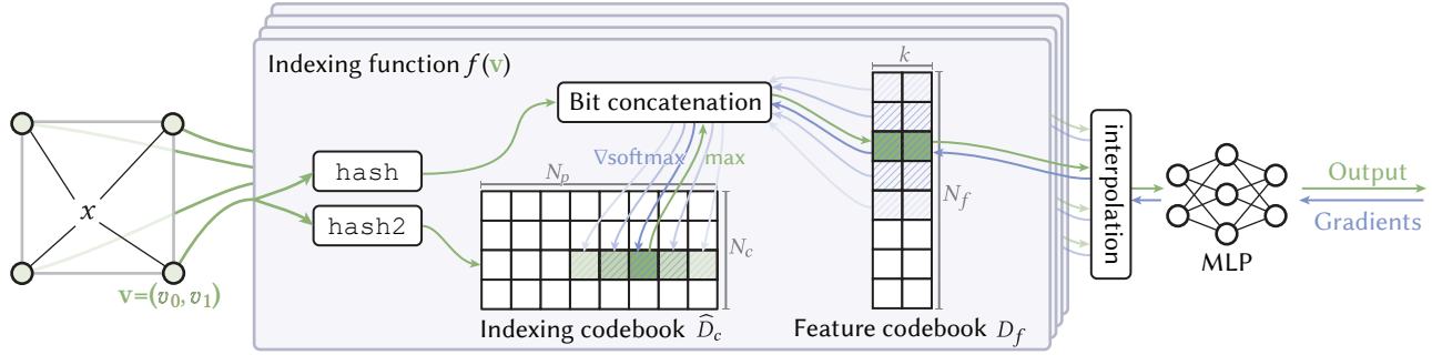
Fig. 4. Overview of Compact NGP. For a given input coordinate \mathbf{x} \in \mathbb{R}^d (far left), we find its enclosing integer grid vertices \mathbf{v} \in \mathbb{Z}^d and apply our indexing function f(\mathbf{v}) to each one. The most significant bits of the index are computed by a spatial hash (hash) and the least significant bits by looking up a row of N_p confidence values from an indexing codebook \widehat{D}_c that is in turn indexed by an auxiliary spatial hash (hash2), and then picking the index with maximal confidence (green arrow). Bitwise concatenation of the two indices yields an index for looking up from the feature codebook D_f , which is subsequently d -linearly interpolated per \mathbf{x} and fed into an MLP. For optimization, we propagate gradients as if the indexing codebook used a softmax instead of a hard maximum, i.e. we use a “straight-through” estimator [Bengio et al. 2013]. In practice, after each training step, we bake this \log_2 N_p -bit indices of the maximal values in each row of \widehat{D}_c into an auxiliary indexing codebook D_c that is both compact and allows for more efficient forward evaluation of the model.
